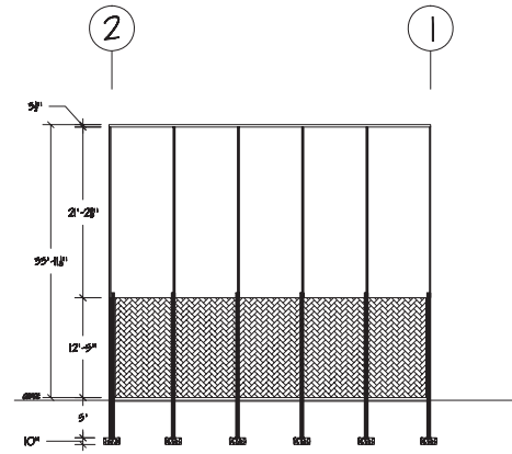
2 5-4 SIDEWALL @ GRID E SCALE: 1/8" = 1'-0"
