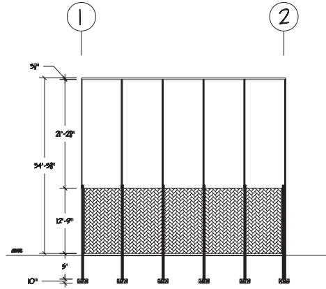
1 5-4 SIDEWALL @ GRID A SCALE: 1/8" = 1'-0"
