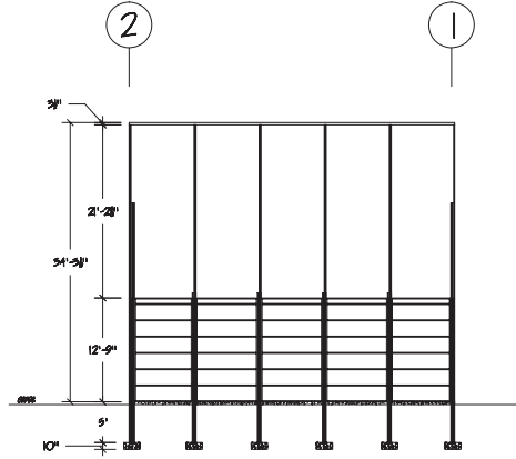
3 5-4 INTERIOR WALL @ GRID B SCALE: 1/8" = 1'-0"
