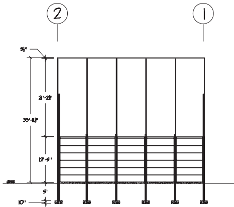
3 5-4 INTERIOR WALL @ GRID D SCALE: 1/8" = 1'-0"
